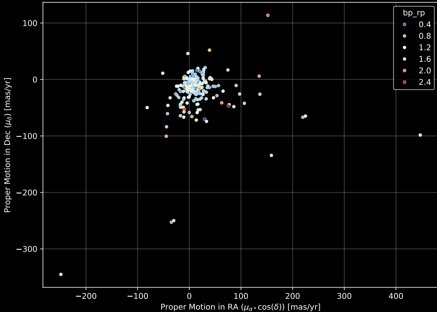
APOGEE DR17 Field: [159-58_MGA] Proper Motion Diagram (n= 214)
