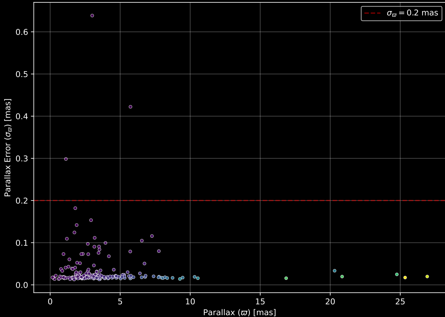
APOGEE DR17 Field: [159-58_MGA] Parallax Quality (n= 214)
