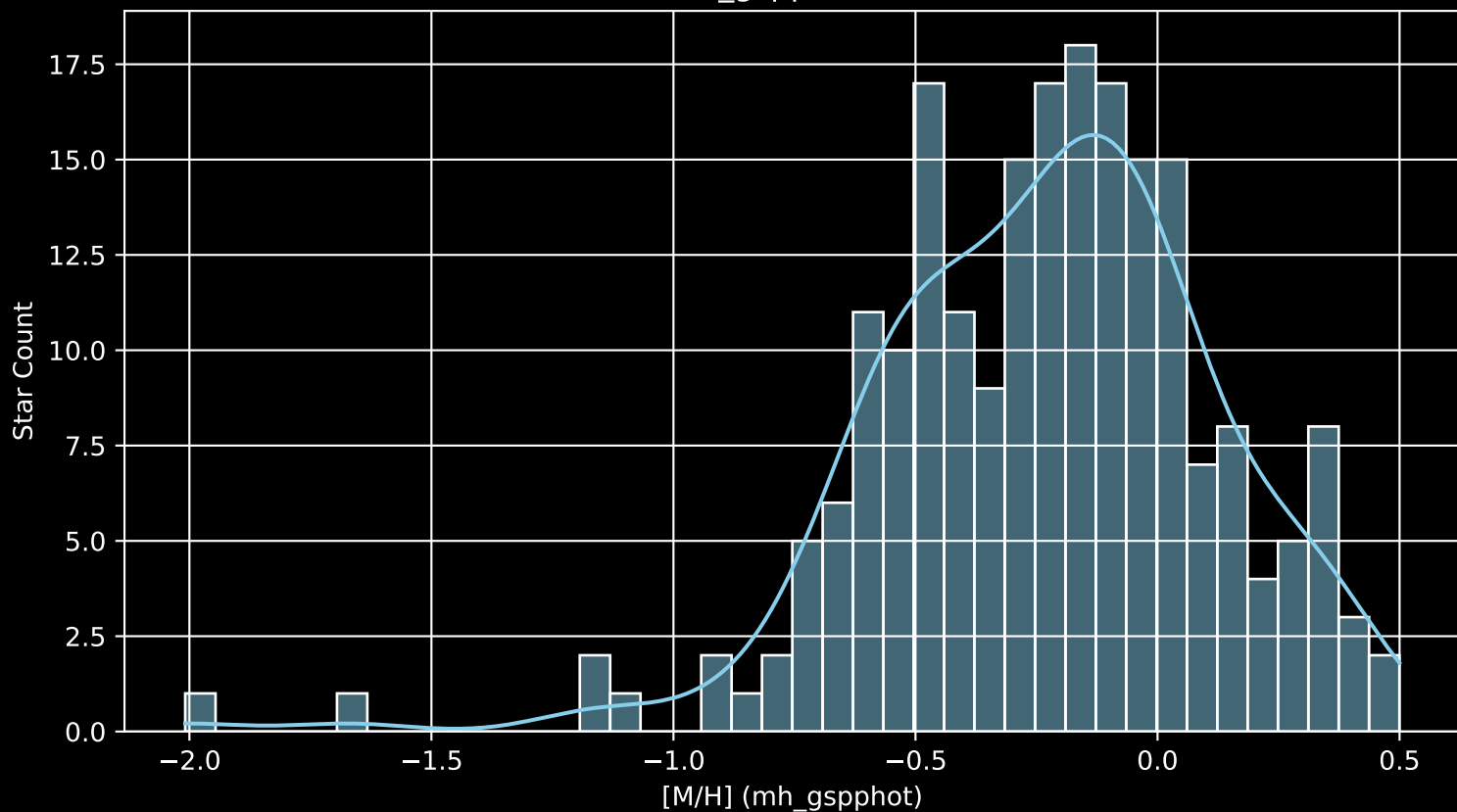
APOGEE DR17 Field: [159-58_MGA [M/H] (mh_gspphot) (n= 213)
