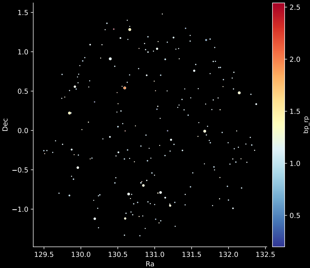
APOGEE DR17 Field: [159-58_MGA] Stars: 214
