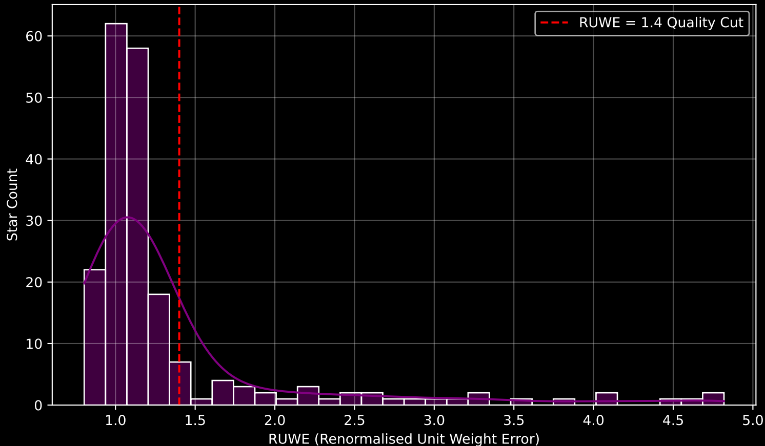
GAPOGEE DR17 Field [159-58_MGA] RUWE Distribution (n= 200)
