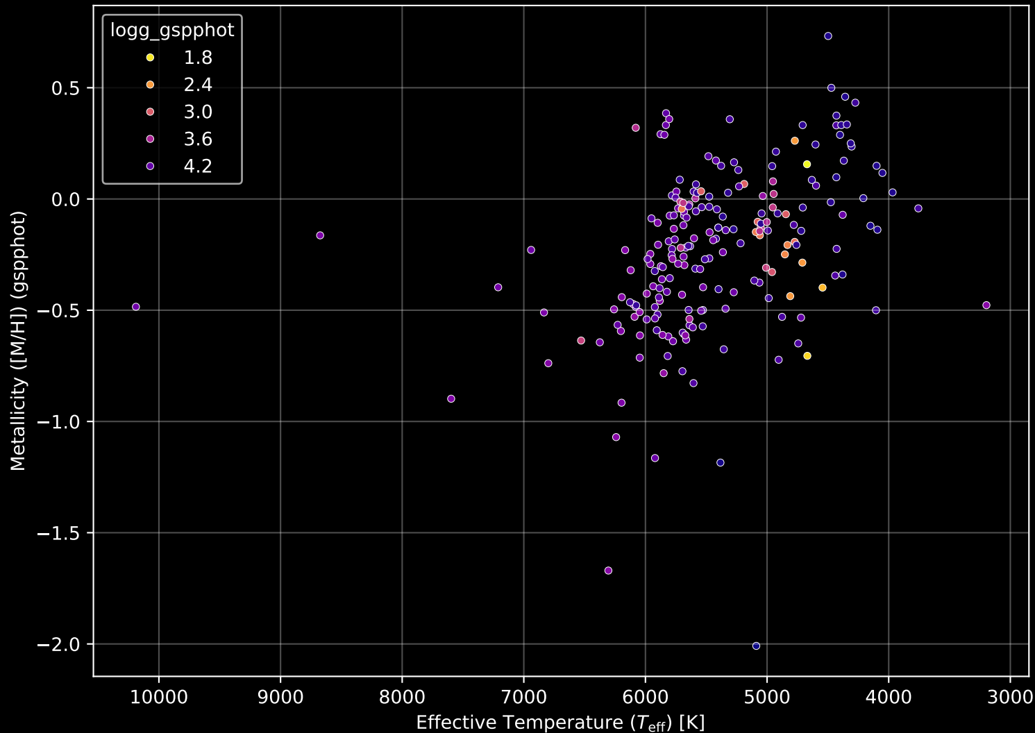
APOGEE DR17 Field: [159-58_MGA] Stellar Population Parameters (n= 214)
